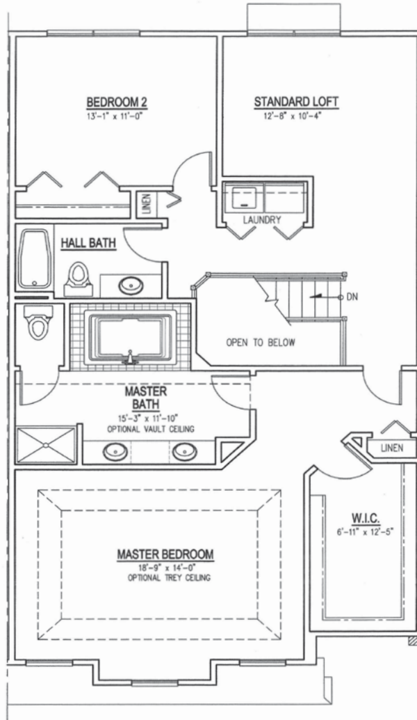
UNIT 'C' - STANDARD SECOND FLOOR PLAN
