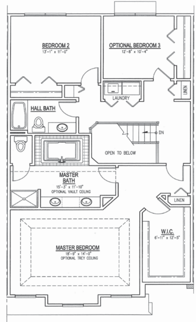
UNIT 'C' - OPTIONAL SECOND FLOOR PLAN
