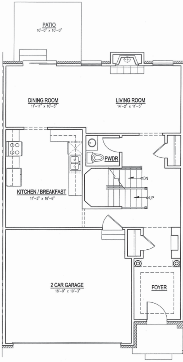
UNIT 'C' - FIRST FLOOR PLAN
