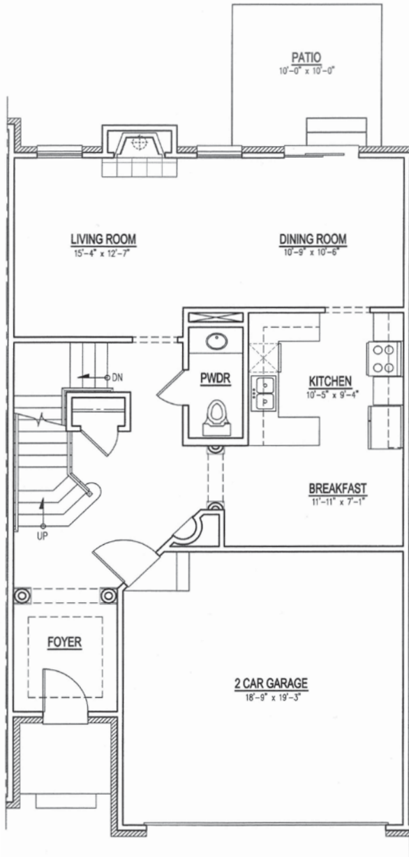
UNIT 'B' - FIRST FLOOR PLAN
