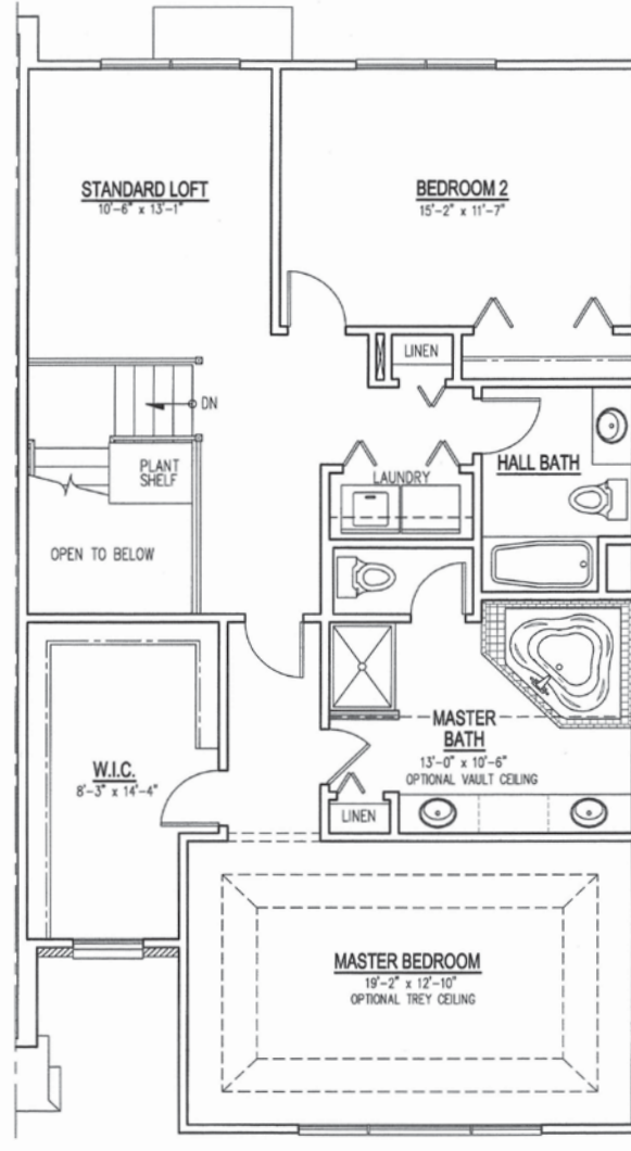
UNIT 'B' - STANDARD SECOND FLOOR PLAN
