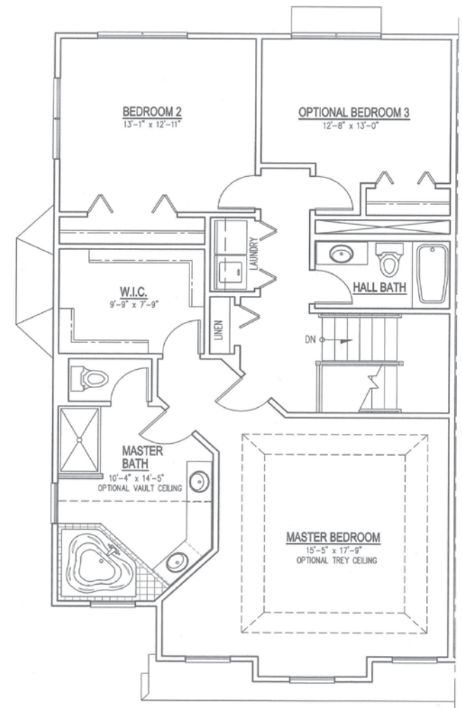
UNIT 'A' - OPTIONAL SECOND FLOOR PLAN
